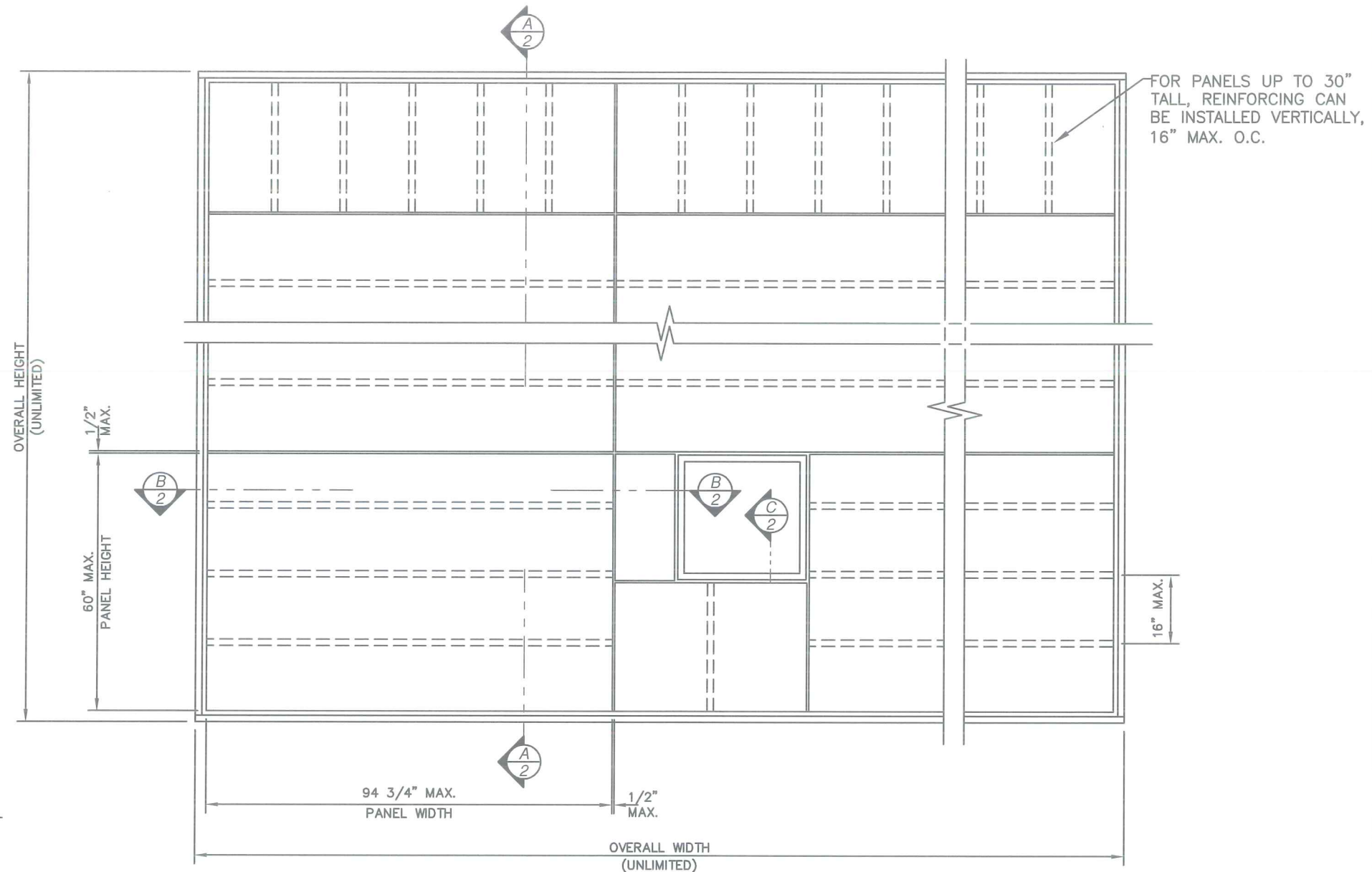
ELEVATION VIEW (FROM EXTERIOR)
